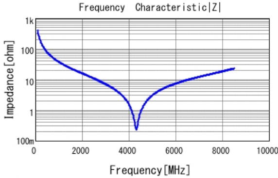
■ GJM1555C1H4R0CB01 |Z| DCOV, 25degC
