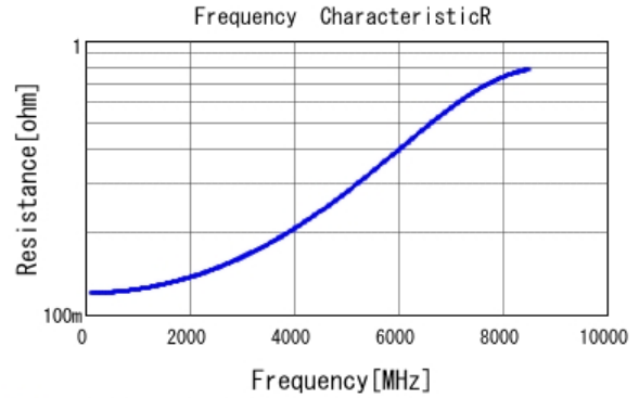
■ GJM1555C1H4R0CB01 R DCOV, 25degC
