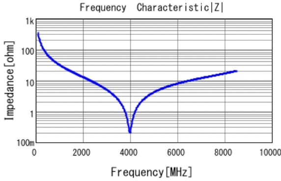
■ GJM1555C1H4R7BB01 |Z| DC0V, 25degC
