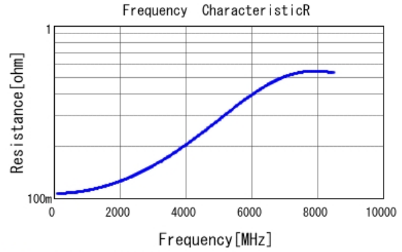
■ GJM1555C1H4R7BB01 R DC0V, 25degC
