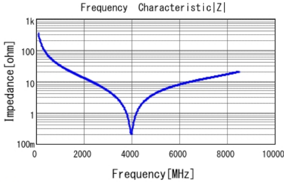
■ GJM1555C1H4R7CB01 |Z| DC0V, 25degC
