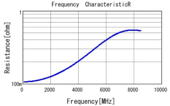
■ GJM1555C1H4R7CB01 R DC0V, 25degC
