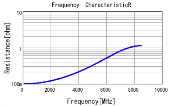
■ GJM1555C1H5R0BB01 R DC0V, 25degC
