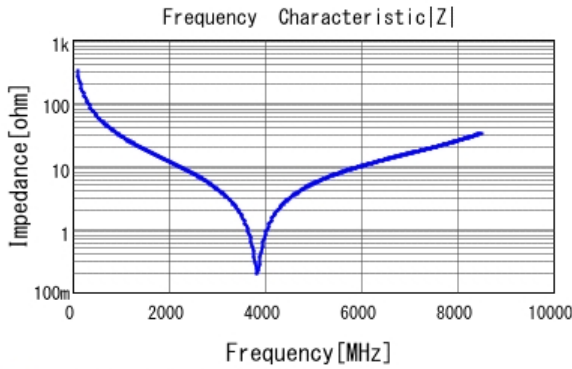
■ GJM1555C1H5R0BB01 |Z| DC0V, 25degC
