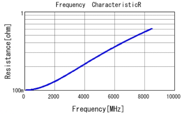
■ GJM1555C1H5R6BB01 R DC0V, 25degC
