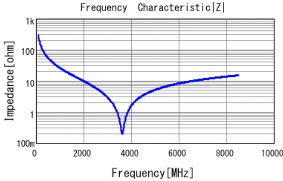
■ GJM1555C1H5R6BB01 |Z| DC0V, 25degC
