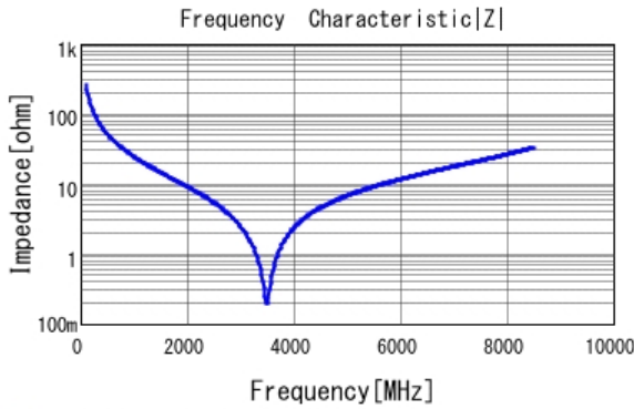
■ GJM1555C1H6R0CB01 |Z| DCOV, 25degC
