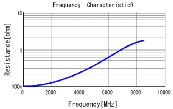
■ GJM1555C1H6R0CB01 R DCOV, 25degC
