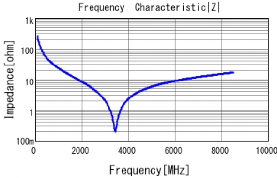
■ GJM1555C1H6R2CB01 |Z| DCOV, 25degC
