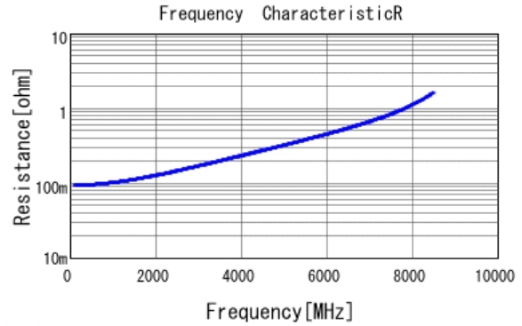
■ GJM1555C1H6R2CB01 R DCOV, 25degC
