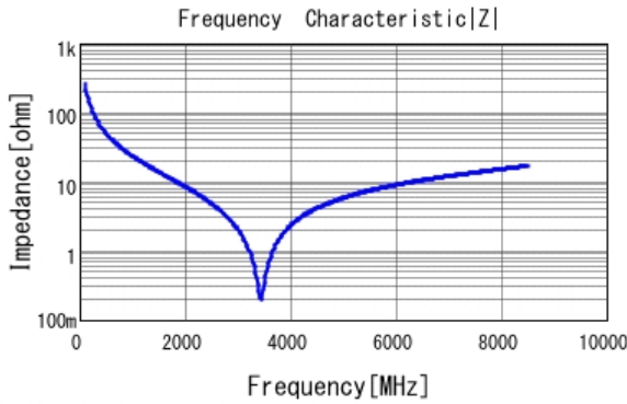
■ GJM1555C1H6R2DB01 |Z| DCOV, 25degC
