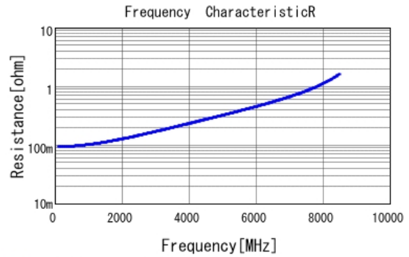
■ GJM1555C1H6R2DB01 R DCOV, 25degC
