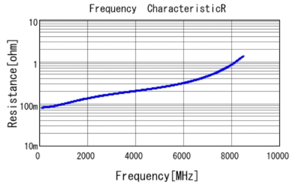
■ GJM1555C1H6R8BB01 R DCOV, 25degC
