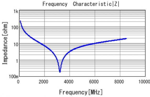
■ GJM1555C1H7R0BB01 |Z| DC0V, 25degC
