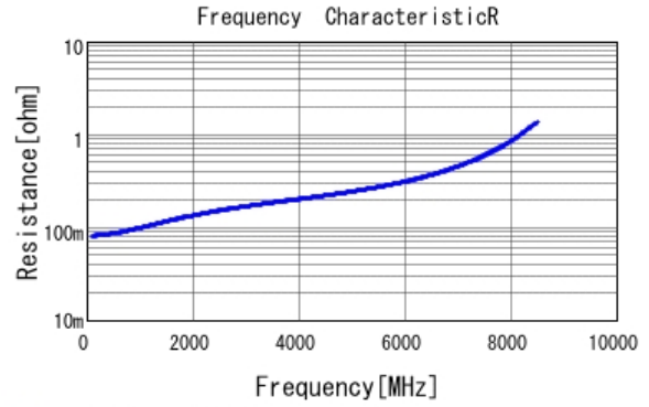
■ GJM1555C1H7R0BB01 R DC0V, 25degC
