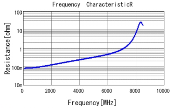
■ GJM1555C1H7R5BB01 R DC0V, 25degC
