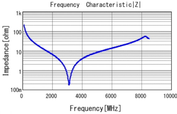
■ GJM1555C1H7R5BB01 |Z| DC0V, 25degC
