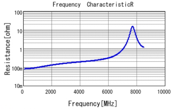
■ GJM1555C1H8R2CB01 R DCOV, 25degC
