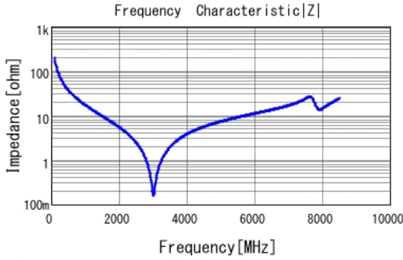
■ GJM1555C1H8R2CB01 |Z| DCOV, 25degC
