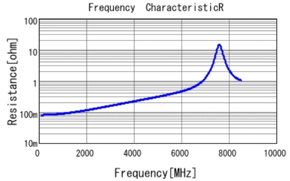
■ GJM1555C1H8R7BB01 R DCOV, 25degC
