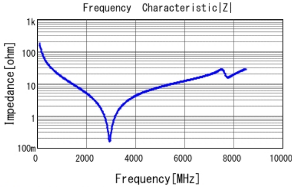
■ GJM1555C1H8R7BB01 |Z| DCOV, 25degC
