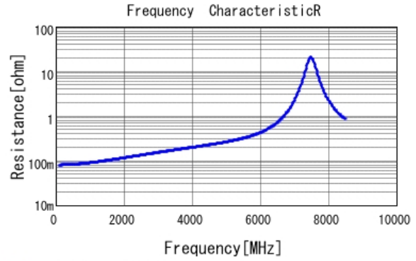
■ GJM1555C1H9R0BB01 R DCOV, 25degC
