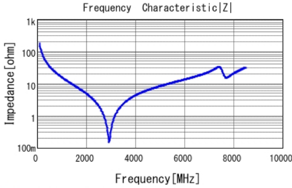
■ GJM1555C1H9R0BB01 |Z| DCOV, 25degC
