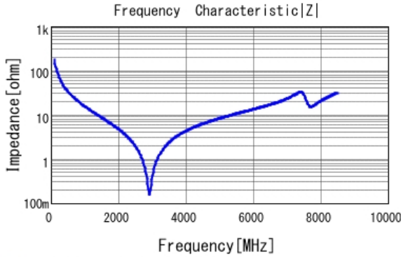
■ GJM1555C1H9R1BB01 |Z| DCOV, 25degC
