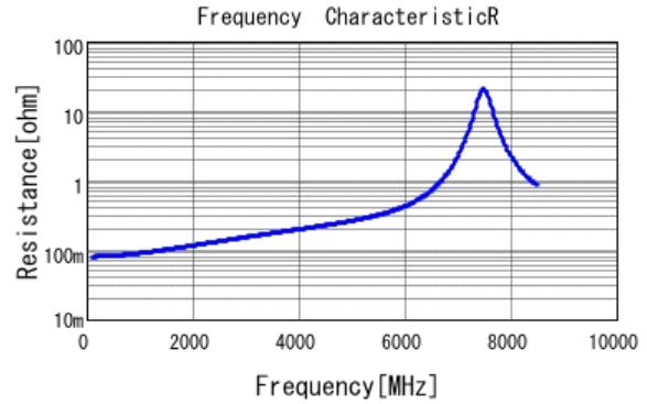
■ GJM1555C1H9R1BB01 R DCOV, 25degC
