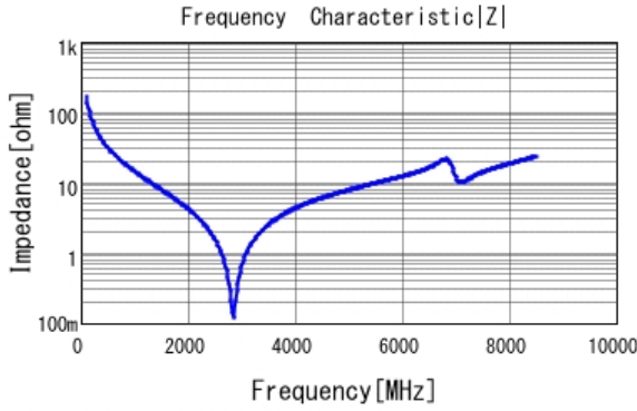
■ GJM1555C1H9R7CB01 |Z| DCOV, 25degC
