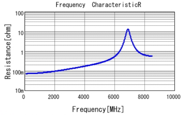
■ GJM1555C1H9R7CB01 R DCOV, 25degC
