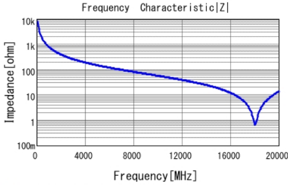
■ GJM1555C1HR20BB01 |Z| DCOV, 25degC
