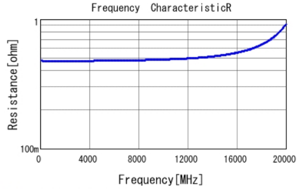
■ GJM1555C1HR20BB01 R DCOV, 25degC
