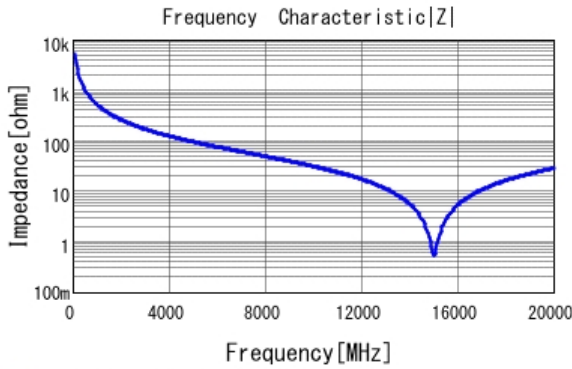
■ GJM1555C1HR30BB01 |Z| DCOV, 25degC
