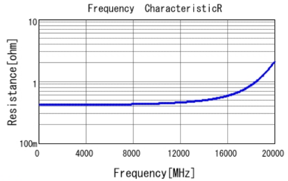
■ GJM1555C1HR30BB01 R DCOV, 25degC
