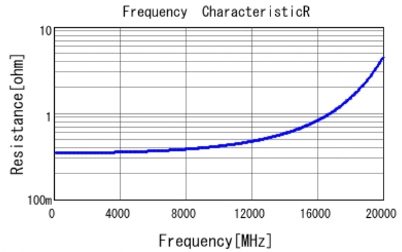
■ GJM1555C1HR40BB01 R DCOV, 25degC
