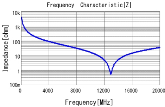
■ GJM1555C1HR40BB01 |Z| DCOV, 25degC
