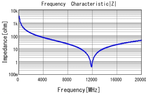
■ GJM1555C1HR50WB01 |Z| DCOV, 25degC
