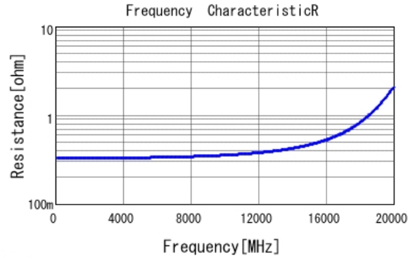
■ GJM1555C1HR50WB01 R DCOV, 25degC
