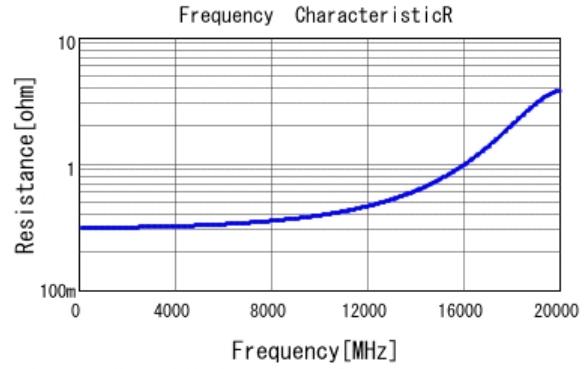
■ GJM1555C1HR60BB01 R DCOV, 25degC
