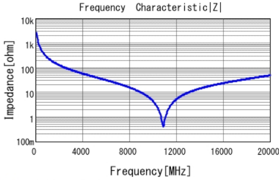
■ GJM1555C1HR60BB01 |Z| DCOV, 25degC
