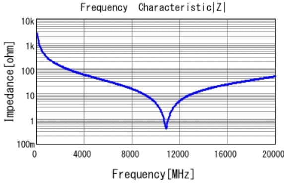
■ GJM1555C1HR60WB01 |Z| DCOV, 25degC
