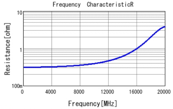
■ GJM1555C1HR60WB01 R DCOV, 25degC
