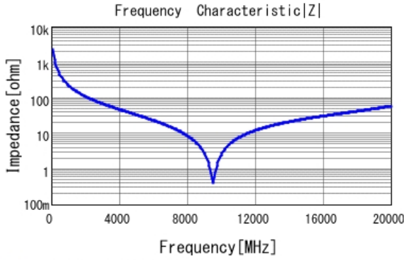
■ GJM1555C1HR70BB01 |Z| DCOV, 25degC
