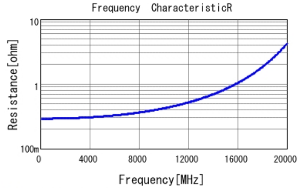
■ GJM1555C1HR70WB01 R DCOV, 25degC
