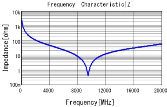
■ GJM1555C1HR70WB01 |Z| DCOV, 25degC
