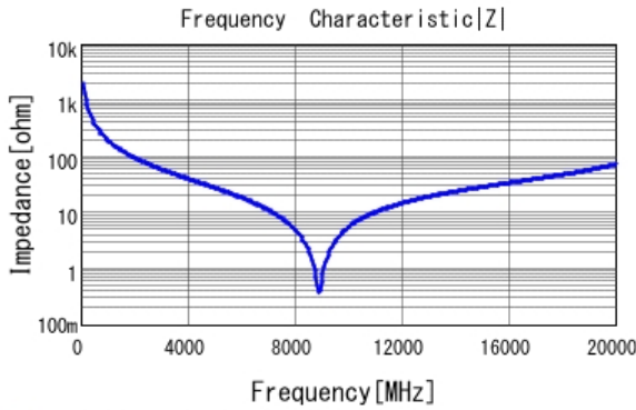
■ GJM1555C1HR80WB01 |Z| DCOV, 25degC
