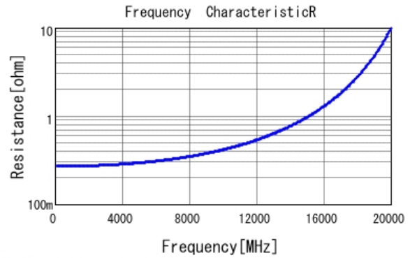
■ GJM1555C1HR80WB01 R DCOV, 25degC
