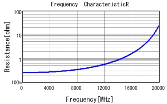
■ GJM1555C1HR90WB01 R DC0V, 25degC
