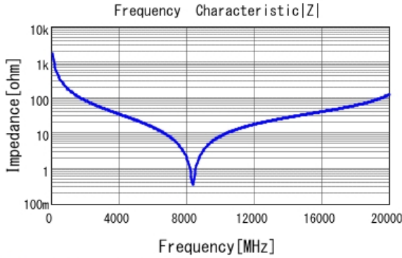
■ GJM1555C1HR90WB01 |Z| DC0V, 25degC
