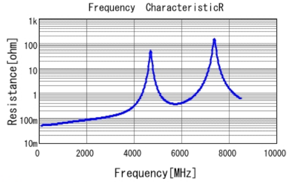
■ GQM1875C2E150GB12 R DC0V, 25degC
