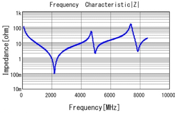
■ GQM1875C2E150GB12 |Z| DC0V, 25degC
