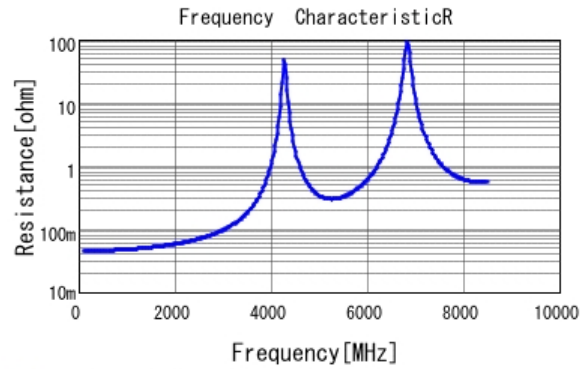
■ GQM1875C2E180JB12 R DCOV, 25degC
