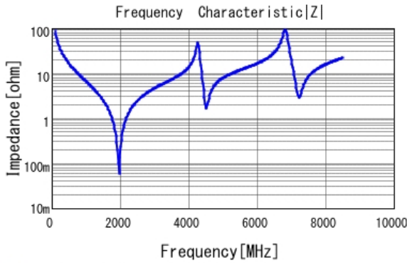
■ GQM1875C2E180JB12 |Z| DCOV, 25degC
