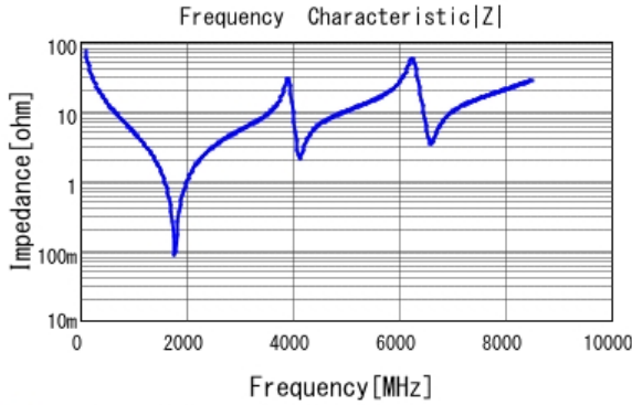
■ GQM1875C2E220JB12 |Z| DCOV, 25degC
