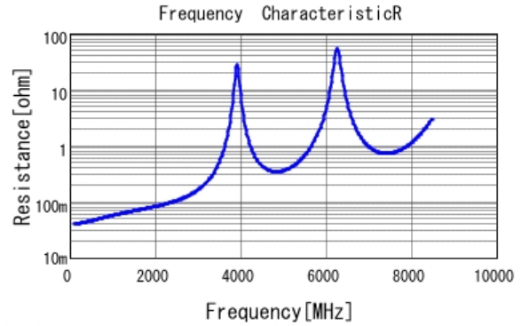
■ GQM1875C2E220JB12 R DCOV, 25degC
