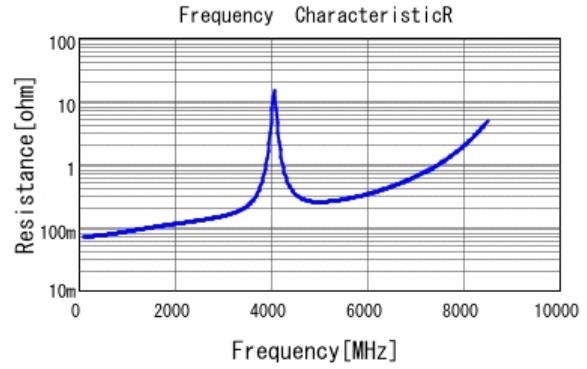
■ GQM1885C1H100GB01 R DCOV, 25degC
