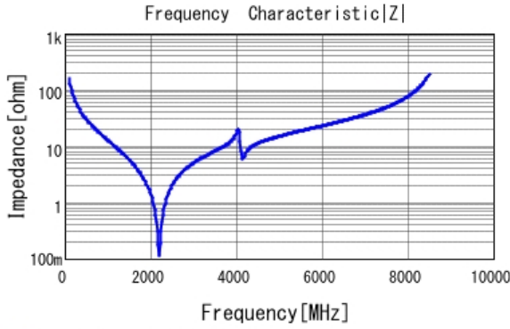
■ GQM1885C1H100GB01 |Z| DCOV, 25degC
