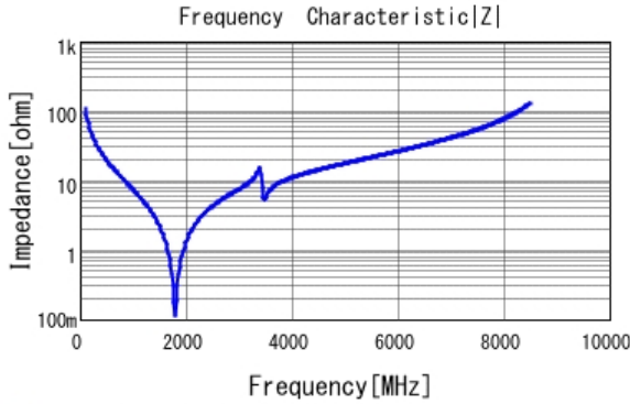
■ GQM1885C1H150GB01 |Z| DCOV, 25degC
