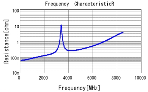
■ GQM1885C1H150GB01 R DCOV, 25degC
