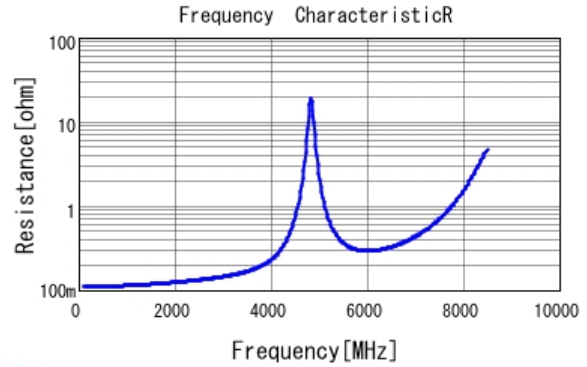
■ GQM1885C1H7R0CB01 R DCOV, 25degC
