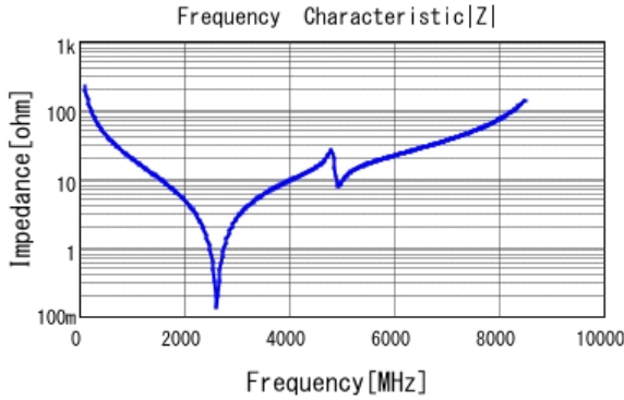
■ GQM1885C1H7R0CB01 |Z| DCOV, 25degC
