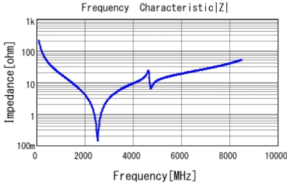
■ GQM1885C1H7R5CB01 |Z| DC0V, 25degC
