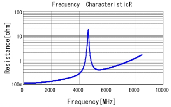
■ GQM1885C1H7R5CB01 R DC0V, 25degC
