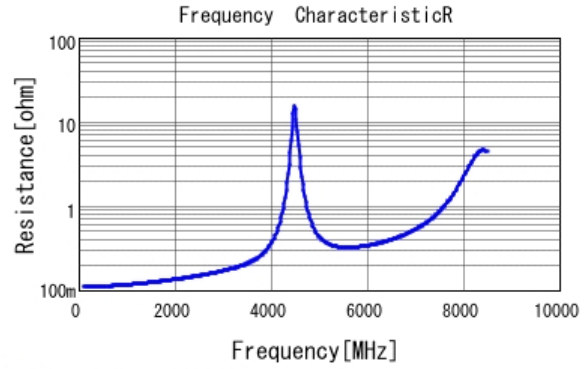
■ GQM1885C1H8R0CB01 R DCOV, 25degC
