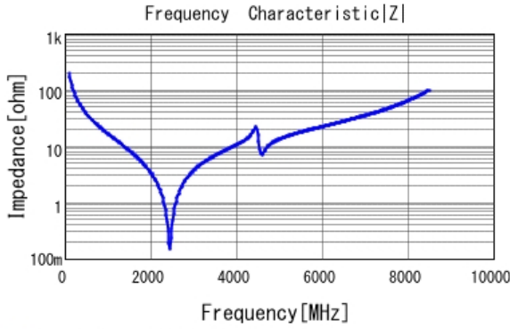
■ GQM1885C1H8R0CB01 |Z| DCOV, 25degC
