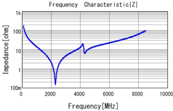
■ GQM1885C1H9R1CB01 |Z| DCOV, 25degC
