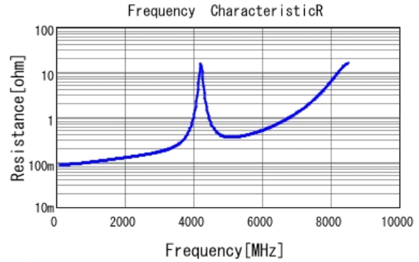
■ GQM1885C1H9R1CB01 R DCOV, 25degC
