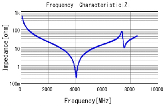
■ GQM1885C2A3R0CB01 |Z| DCOV, 25degC
