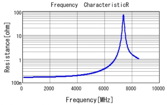
■ GQM1885C2A3R0CB01 R DCOV, 25degC
