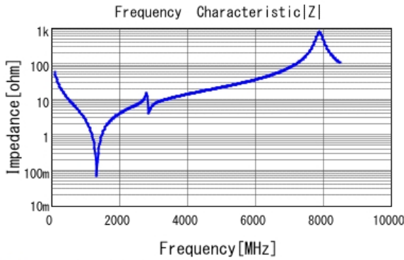
■ GQM2195C1H270JB01 |Z| DCOV, 25degC
