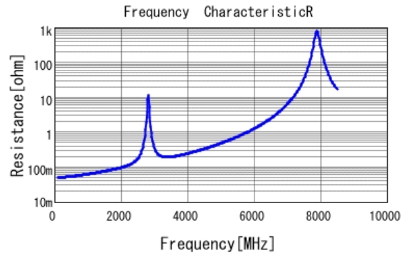
■ GQM2195C1H270JB01 R DCOV, 25degC
