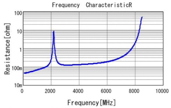
■ GQM2195C1H470JB01 R DCOV, 25degC
