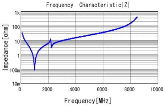
■ GQM2195C1H470JB01 |Z| DCOV, 25degC
