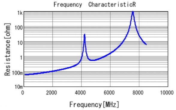
■ GQM2195C2A120JB01 R DC0V, 25degC
