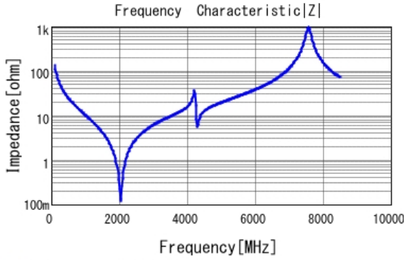
■ GQM2195C2A120JB01 |Z| DC0V, 25degC
