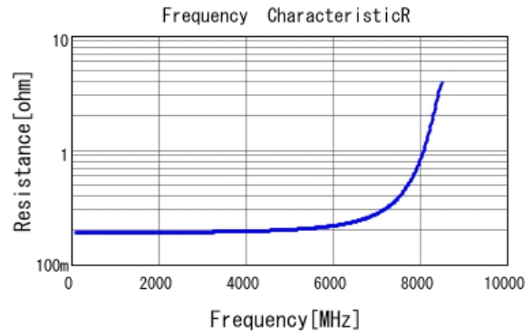
■ GQM2195C2A1R2BB01 R DC0V, 25degC
