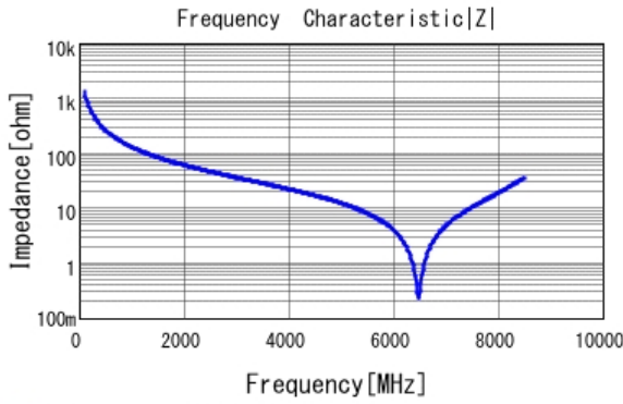
■ GQM2195C2A1R2BB01 |Z| DC0V, 25degC
