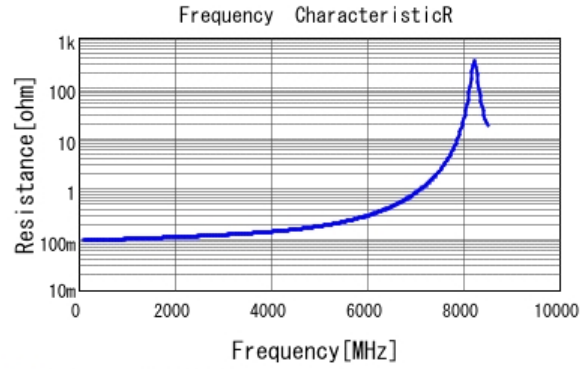
■ GQM2195C2A2R7BB01 R DCOV, 25degC
