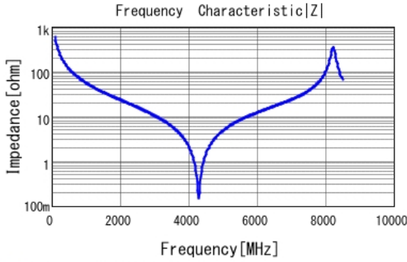
■ GQM2195C2A2R7BB01 |Z| DCOV, 25degC
