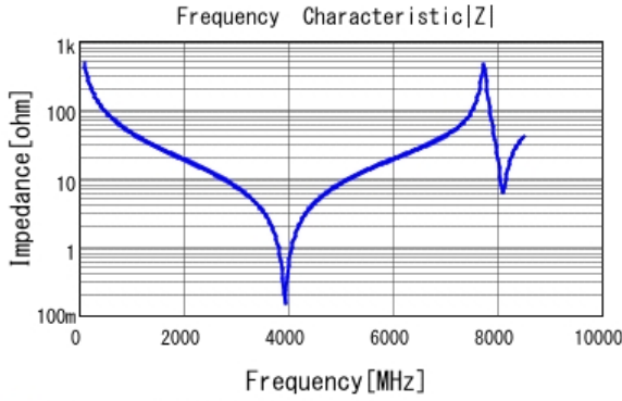
■ GQM2195C2A3R3BB01 |Z| DCOV, 25degC
