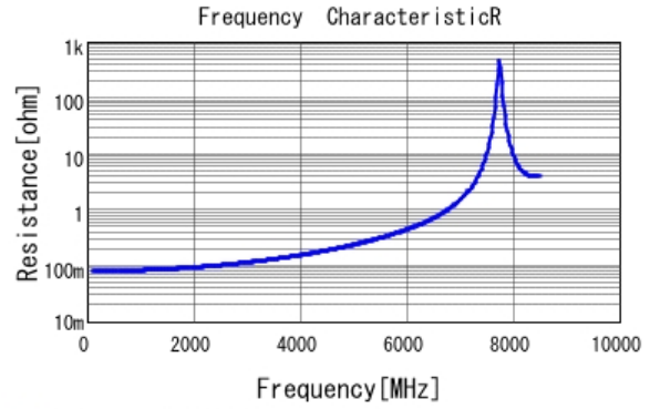
■ GQM2195C2A3R3BB01 R DCOV, 25degC
