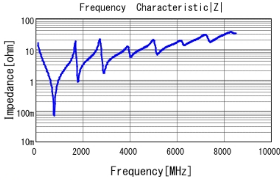
■ GQM2195C2E101GB12 |Z| DC0V, 25degC
