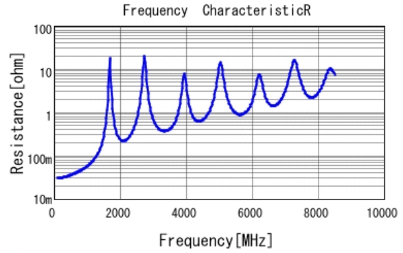
■ GQM2195C2E101GB12 R DC0V, 25degC
