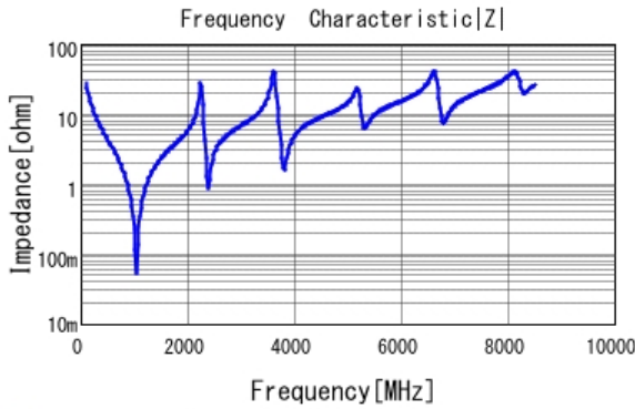
■ GQM2195C2E560JB12 |Z| DCOV, 25degC
