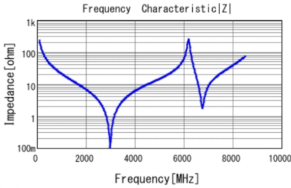
■ GQM2195C2E6R8CB12 |Z| DCOV, 25degC
