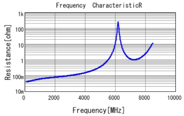
■ GQM2195C2E6R8CB12 R DCOV, 25degC
