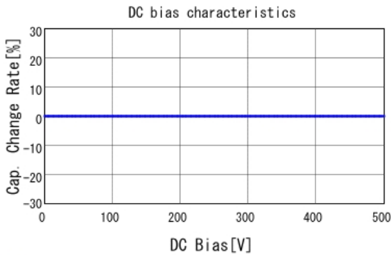
■ GQM22M5C2H101JB01 C-DC bias capchange, 25.0degC, AC1V
