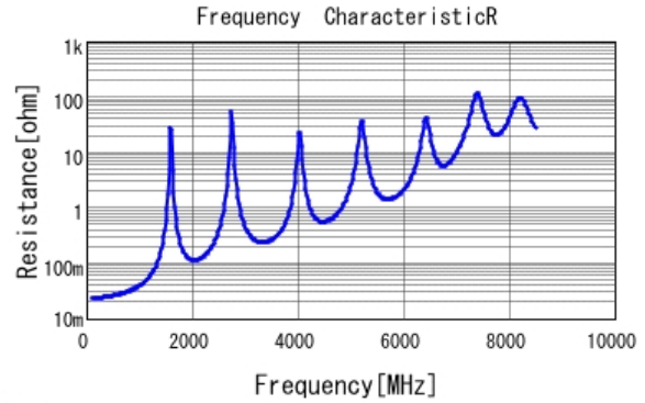
■ GQM22M5C2H101JB01 R DC0V, 25degC
