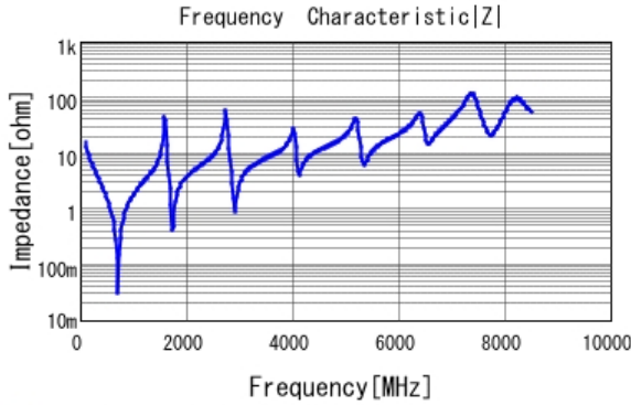
■ GQM22M5C2H101JB01 |Z| DC0V, 25degC
