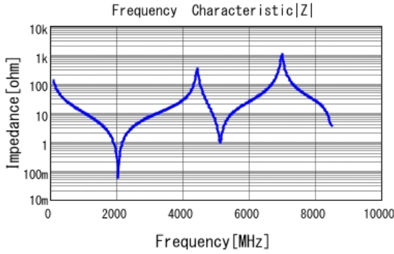
■ GQM22M5C2H120JB01 |Z| DC0V, 25degC
