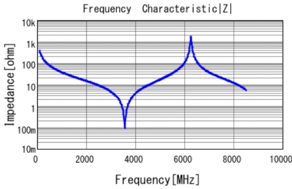
■ GQM22M5C2H4R0CB01 |Z| DC0V, 25degC
