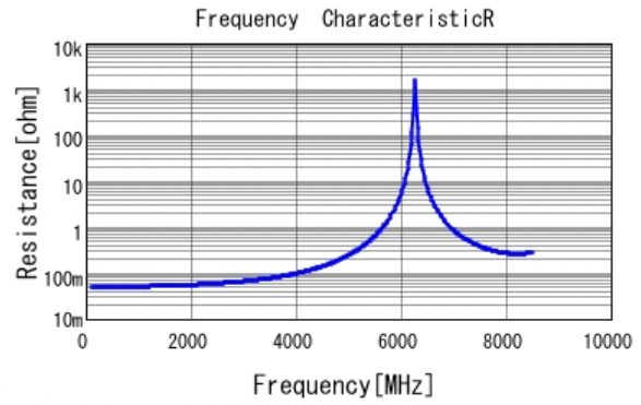
■ GQM22M5C2H4R0CB01 R DC0V, 25degC
