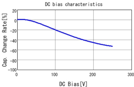
■ GR321AD72E103KW01 C-DC bias capchange, 25.0degC, AC1V
