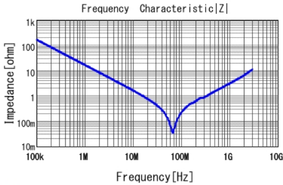
■ GR321AD72E103KW01 |Z| DC0V, 25degC
