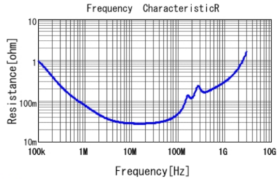
■ GR321AD72E103KW01 R DC0V, 25degC
