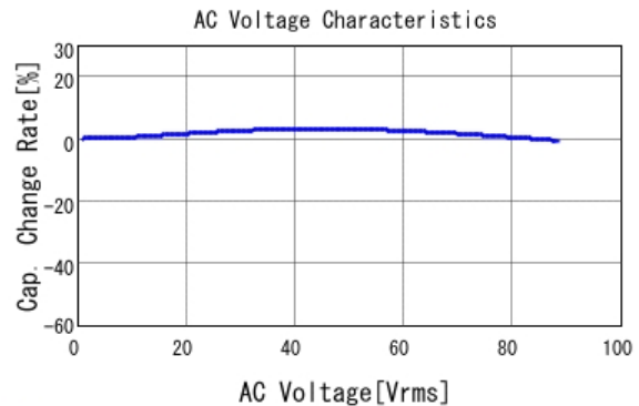
■ GR321AD72E103KW01 C-AC Voltage capchange, DC0V, 25.0d
