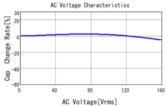
■ GR332DD72W104KW01 C-AC Voltage capchange, DC0V, 25.0d
