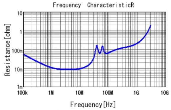
■ GR332DD72W104KW01 R DC0V, 25degC
