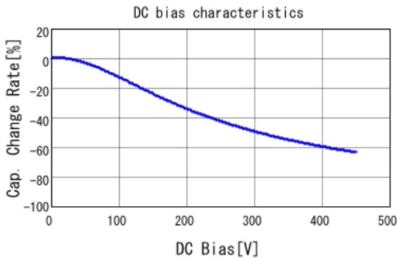
■ GR332DD72W104KW01 C-DC bias capchange, 25.0degC, AC1V
