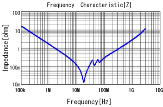
■ GR332DD72W104KW01 |Z| DC0V, 25degC
